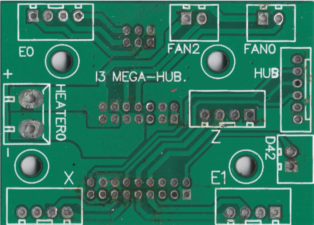
distribution circuit board, outside (REVERSED)
